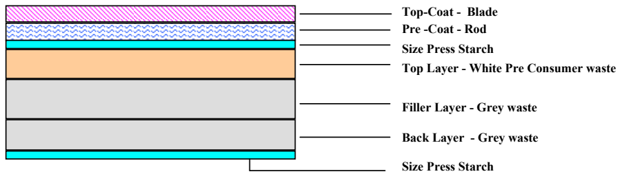
CBGB - HS Board Structure
